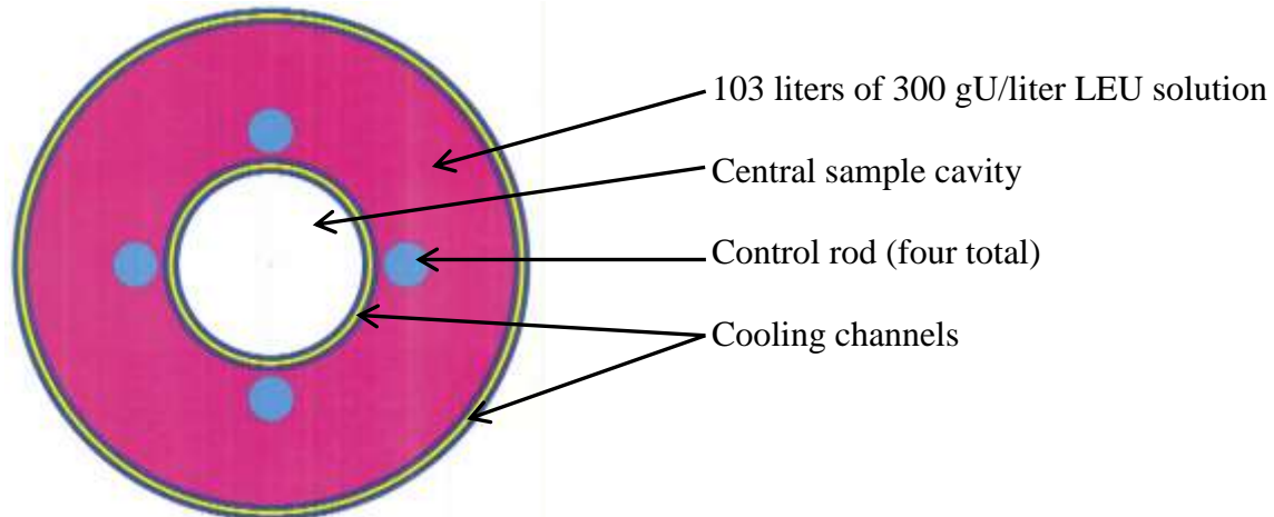
Figure 1: Annular Core AHR with Cooling Channels
