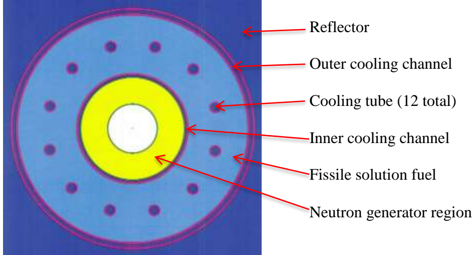
Figure 3: Notional Accelerator-Driven Sub-Critical Assembly
